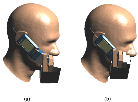
Fig. 5 The SEMCAD X representation of; (a) Model-C in hand1 against SAM at check position, (b) Model-C in hand2 against SAM at check position
