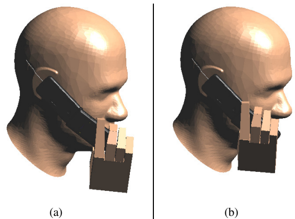
Fig. 6 The SEMCAD X representation of; (a) Model-D in hand1 against SAM at check position, (b) Model-D in hand2 against SAM at check position
