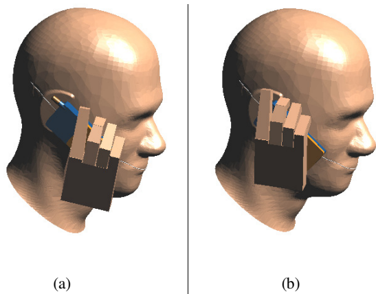
Fig. 3 The SEMCAD X representation of; (a) Model-A in hand1 against SAM at check position, (b) Model-A in hand2 against SAM at check position
