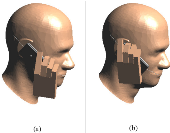
Fig. 4 The SEMCAD X representation of; (a) Model-B in hand1 against SAM at check position, (b) Model-B in hand2 against SAM at check position
