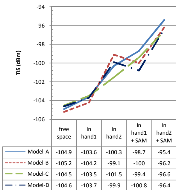
Fig. 8 TIS versus mobile phone setup for the different adopted models at 900 MHz
