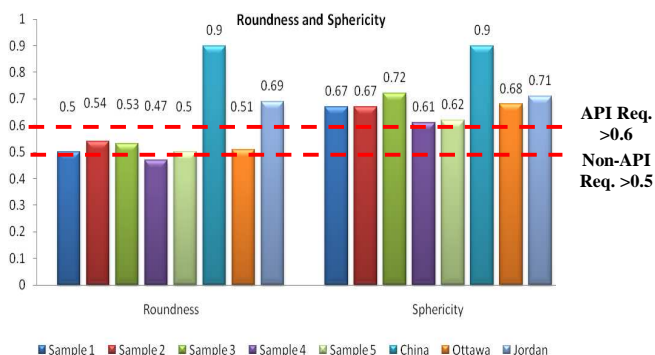
Fig. 5 Roundness and Sphericity Comparative Graph
