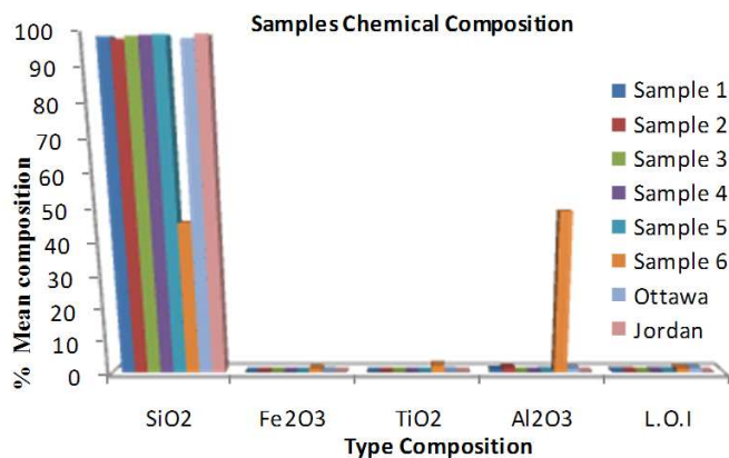
Fig. 7 Chemical Composition Comparative Graph
