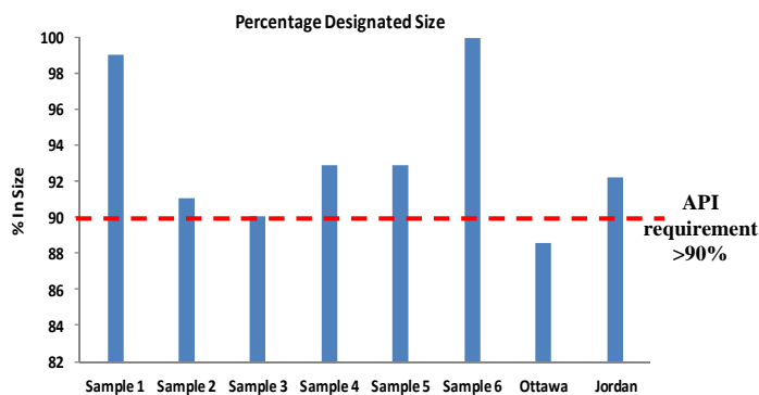
Fig. 3 Percentage designated in size comparative graph
