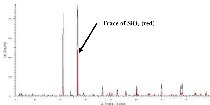
Fig. 8 XRD Analysis of Sample 6, Sample 1 and Sample 2
