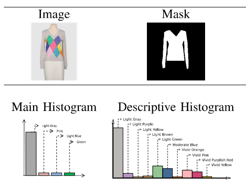
Fig. 2 An example of colors extracted from an offer's image in according to the set of pixel belonging to the object of interest showed in the alpha mask. The histogram represents the amount of colors contained in the object of interest. For each histogram's bin the textual descriptor of the representative colors is displayed.
