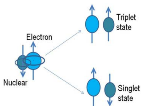
Fig. 2. The hyperfine interaction.
