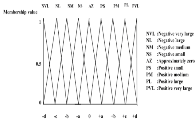
Fig. 1 The membership function of the fuzzy output.
