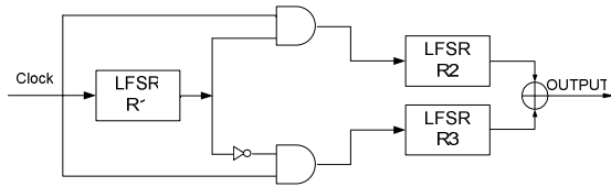
Fig. 4 Clock control generator
