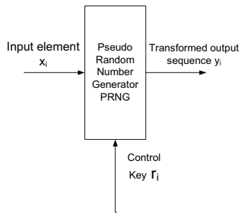
Fig. 5 Stochastic transformation
