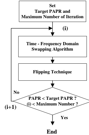
Fig. 5 Flow chart of proposed algorithm
