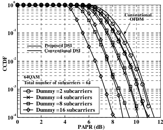
Fig. 6 PAPR performance of proposed DSI method
