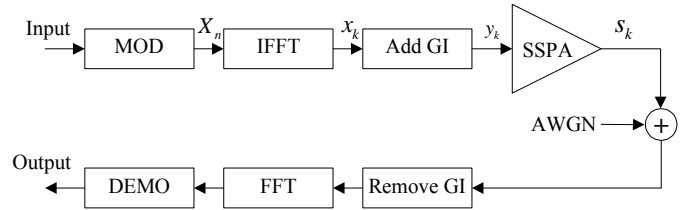
Fig. 1 Block diagram of OFDM system
