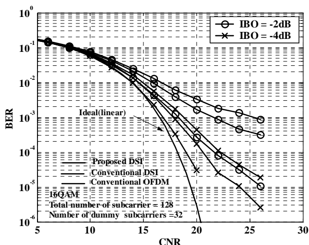
(a) 16QAM
