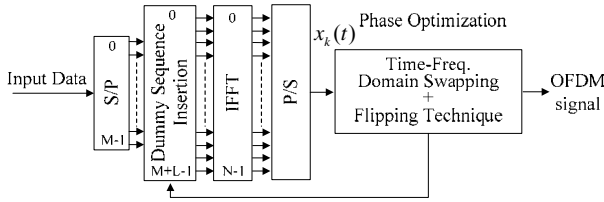
Fig. 4 Block diagram of phase optimization method
