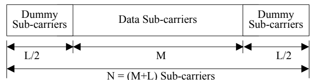
Fig. 3 Structure of proposed OFDM symbol
