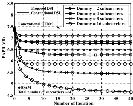
Fig. 7 PAPR performance versus number of iterations
