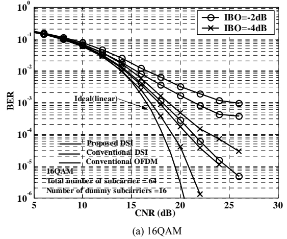
(a) 16QAM
