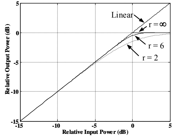
Fig. 2 Input-output relationship of SSPA
