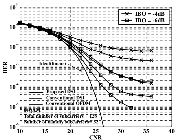
(b) 64QAM
