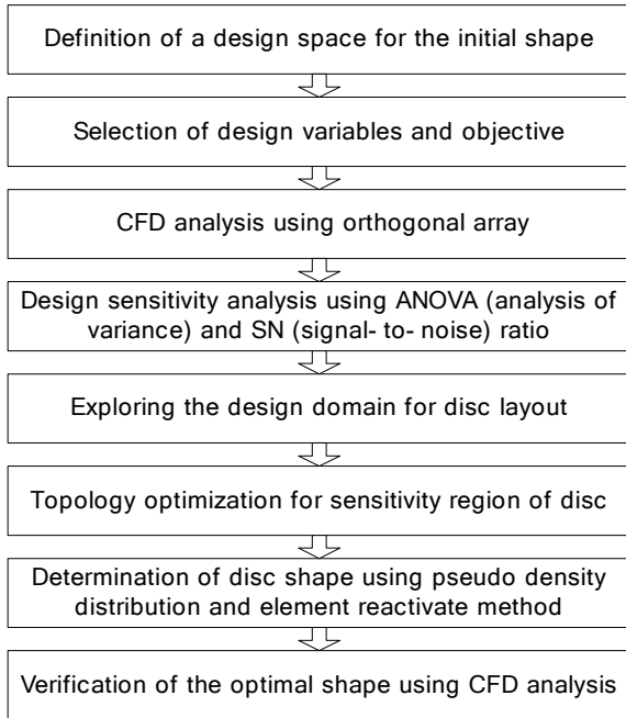
Fig. 4 Flowchart of the valve disc optimization procedure
