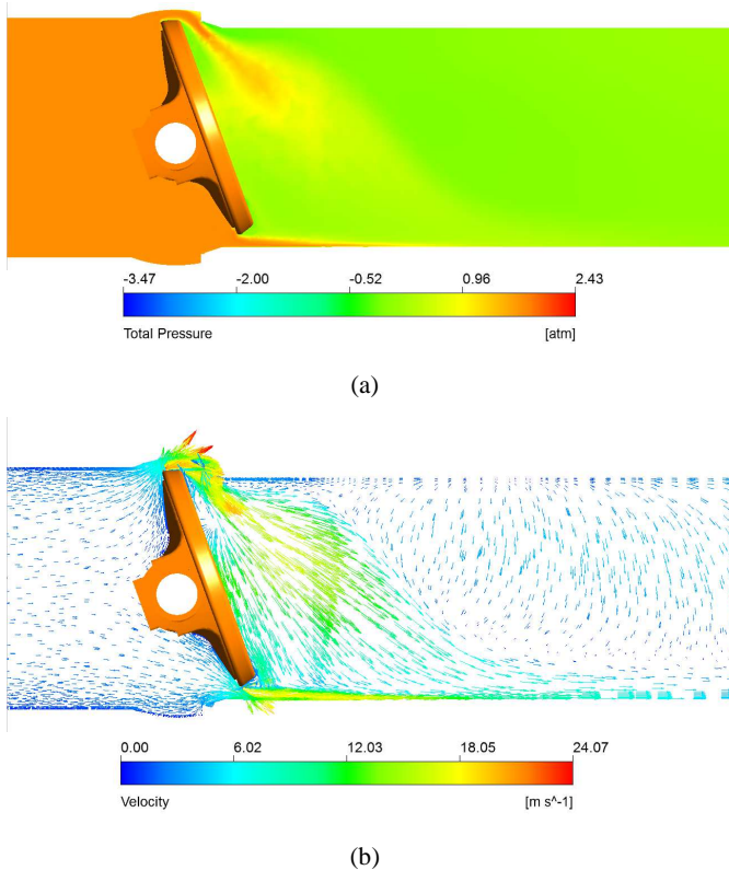
Fig. 3 CFD results of valve disc at 20° opening, (a) pressure, (b) velocity magnitude
