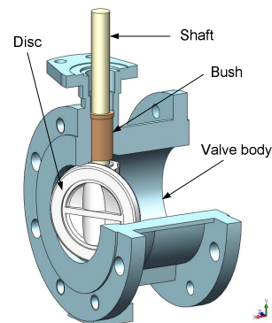
Fig. 1 Overall structure of a double-eccentric butterfly valve
