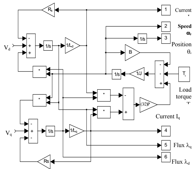
Fig. 2 Simulated motor in the d-q reference frame
