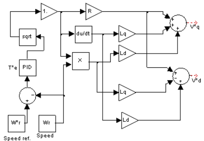
Fig. 5 The voltage reference controller block diagram
