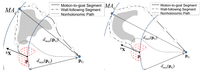
Fig. 9 Second case: the robot cannot see the both paths to points \mathbf{P}_R, \mathbf{P}_L . The some part of blocking obstacle is included within the circle radius d_{min}(\mathbf{p}_G) (left) or not (right) at the switching point to the motion-to-goal behavior
