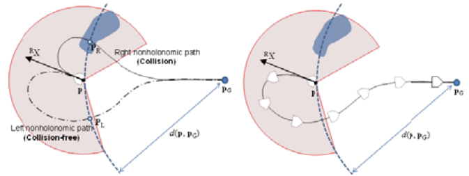
Fig. 8 Fist case: the robot can see the both paths to points \mathbf{P}_R, \mathbf{P}_L . After the nonholonomic path is determined (left), the robot follows the nonholonomic path (right)
