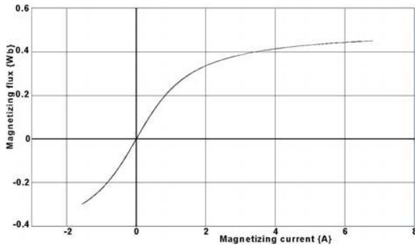
Fig. 5. Nonlinear performance of the transformer of Fig. 3.
