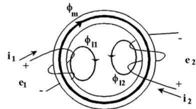
Fig. 2. Magnetic coupling of a two-winding transformer.
