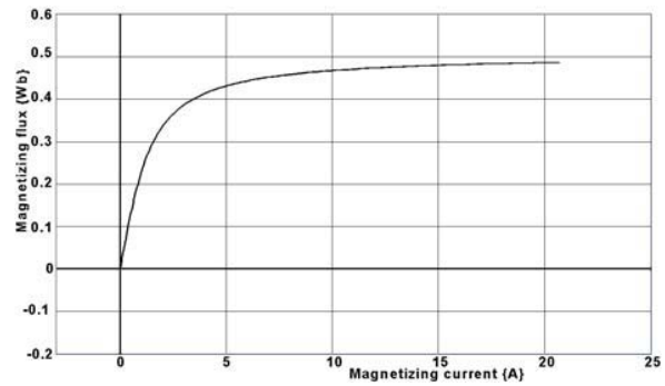
Fig. 4. Saturation curve of equation (49).
