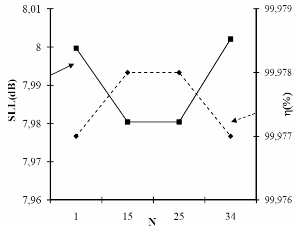
Fig. 7 SLL(\text{dB}) and \eta(\%) variations at f=80\text{GHz} versus N for N_{\text{strip}}=25 ( L_0 \approx 17\lambda_0 ), b(1)/C=\Delta b/C=0.5 , \epsilon_r=2.5 , C=0.734\lambda_0 , a=0.32\lambda_0 , W=0.3307\lambda_0 , d=0.667\lambda_0 . ( \lambda_0=3.75\text{mm} at f_0=80\text{GHz} )
