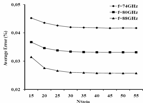
Fig. 3 Comparison between the approximated and the exact methods. The representation of the average error (%) versus the frequency f(\text{GHz}) and the number of strips N_{\text{strip}} in millimeter band. \epsilon_r=2.5 , b=C=0.734\lambda_0 , a=0.32\lambda_0 , d=0.667\lambda_0 , W=0.3307\lambda_0 . ( \lambda_0=3.75\text{mm} à f=80\text{GHz} ).
