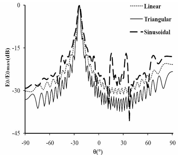
Fig. 8 Comparison between normalized radiating patterns E_{\theta}/E_{\theta\max}(\text{dB}) at f=80\text{GHz} . \epsilon_r=2.5 , C=0.734\lambda_0 , a=0.32\lambda_0 , W=0.3307\lambda_0 , d=0.667\lambda_0 . ( \lambda_0=3.75\text{mm} at f_0=80\text{GHz} )
