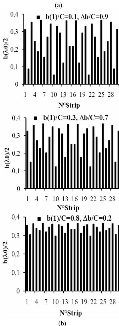
Fig. 6 (a) Normalized radiating patterns E_{\theta}/E_{\theta\max} (dB) for N=19 and N_{\text{strip}}=30 ( L_0 \approx 20\lambda_0 ) at f=80\text{GHz} . (b) Sinusoidal distributions b(\lambda_0)/2 of metallic strips. \epsilon_r=2.5 , C=0.734\lambda_0 , a=0.32\lambda_0 , W=0.3307\lambda_0 , d=0.667\lambda_0 . ( \lambda_0=3.75\text{mm} at f_0=80\text{GHz} ).
