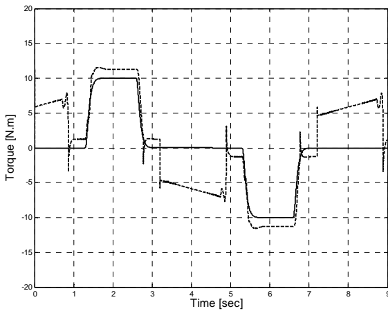
Fig. 12. Motor and load torques
