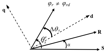
Fig.1: Representative diagram of the loss of decoupling
