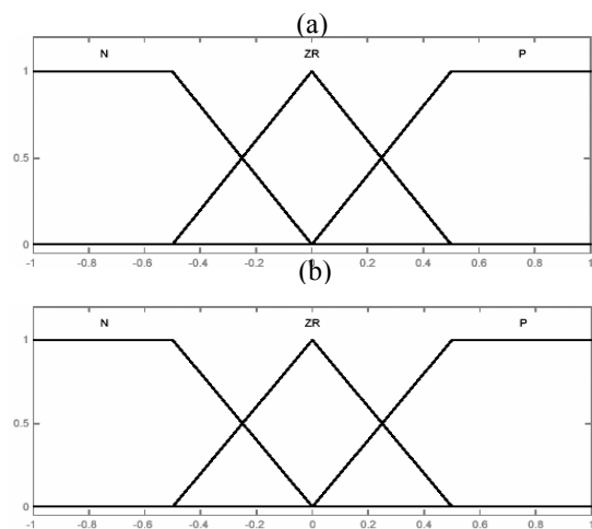
Fig.4: Input and output membership functions (a): e_{\Omega 1} , (b): \Lambda e_{\Omega 1}
