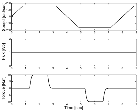
Fig. 6. Reference trajectories
