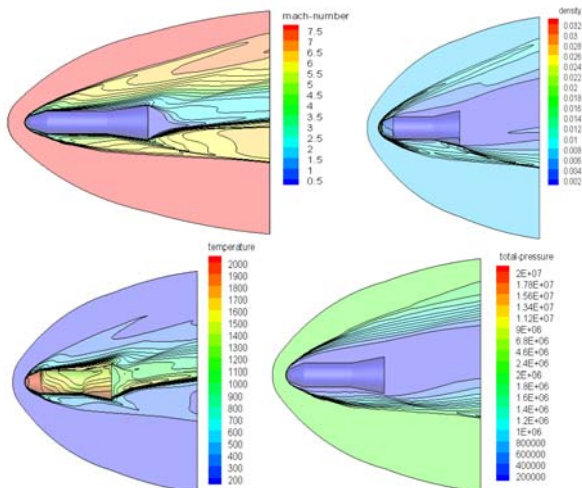
Fig: 10 frustrum 10° contours of Mach number density temperature and total pressure at mach 8 angle of attack 8°
