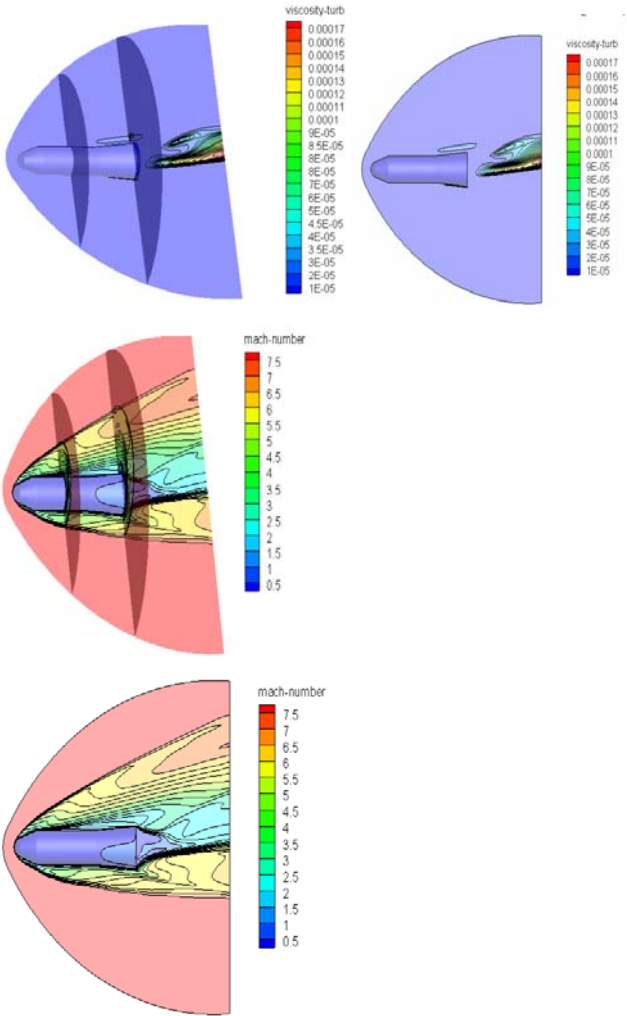
Fig: 7 cone-cylinder frustrum 5 deg DES and SA Model contours of turbulent viscosity Mach (at mach 8 angle of attack 10°)
