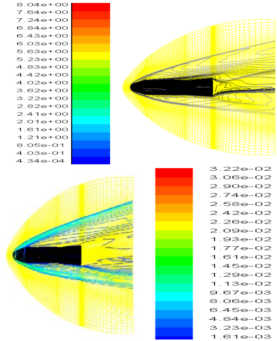
Fig. 8 cone-cylinder frustrum 5° contours of Mach number, density, at mach 8 and angle of attack 6° for DES
