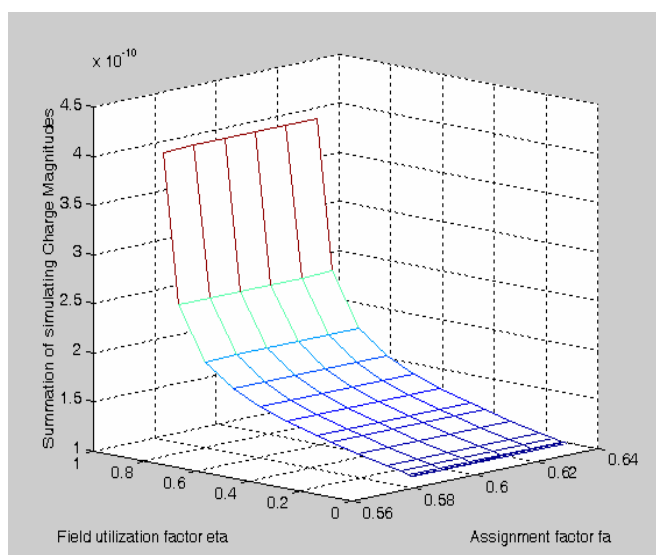
Fig. 6 Plot of summation of simulating charges of the sphere as a function of assignment factor 'fa' for selected values of field utilization factor 'η' over its entire range (six-point-charge model).
