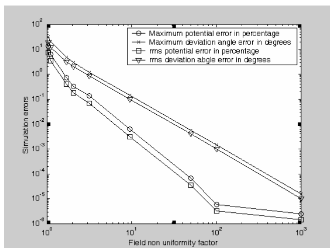
Fig. 8 CSM simulation errors as a function of non uniformity factor (with optimal assignment factor based charge locations) for sphere plane gap (with six-point-charge model).
