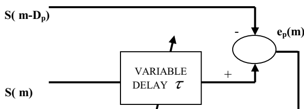
Fig. 1 Tracking time delay algorithm configuration
