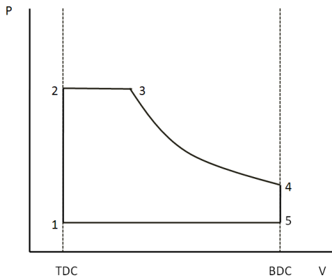
Fig. 4 P-V diagram for the pneumatic motoring cycle
