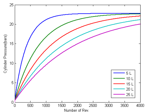
Fig. 3 Air compression pumping
