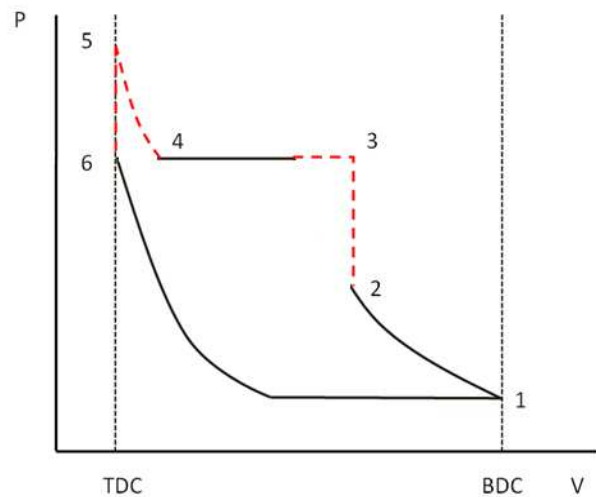
Fig. 2 P-V diagram of pneumatic pump operation
