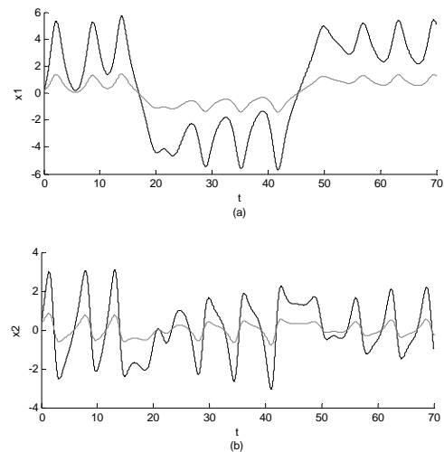
Fig.6 Synchronization of the fractional-order chaotic Duffing systems (21) and (22) with K = (1.85, 1.7225), \sigma = 4 . (a) x_1, \tilde{x}_1 ; (b) x_2, \tilde{x}_2 .
