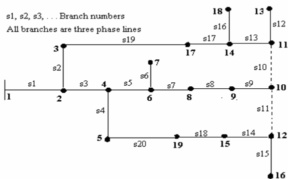
Fig. 4 Single line diagram of 19 node URDS after network reconfiguration
