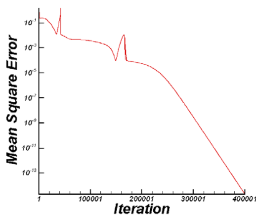
Fig. 4 Roughness ANN learning convergence
