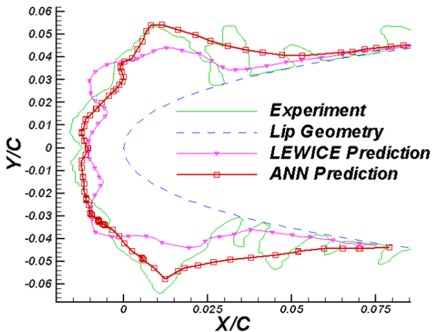
Fig. 5 Glaze ice shape on intake lip geometry
