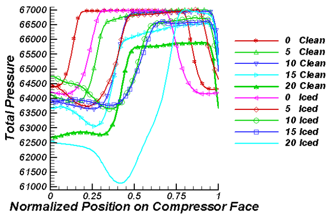
Fig. 7 Total pressure (Pa) variations across compressor face at different AOAs
