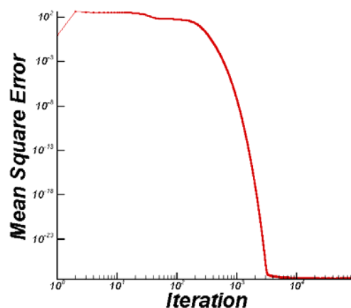
Fig. 2 X-coefficient ANN learning convergence
