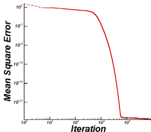
Fig. 3 Y-coefficient ANN learning convergence
