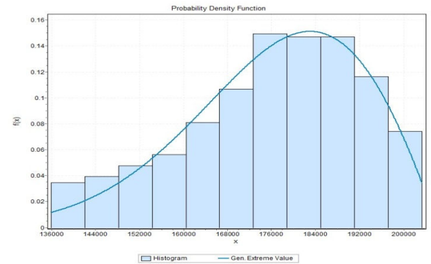
Fig. 7 Histogram of traffic during peak-load hours at Switch S13
