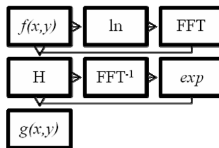
Fig. 5 The process of homomorphic filtering
