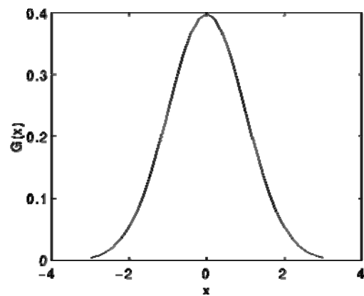
Fig. 1 1-D Gaussian distribution (mean=0 standard deviation=1)
