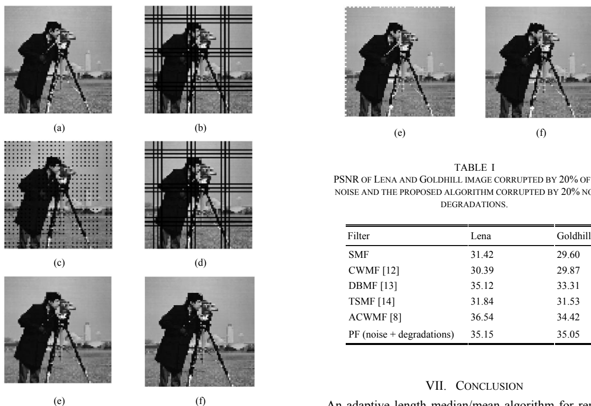
Fig. 6: Drop lines removal. (a) Original image. (b) Corrupted by drop lines. (c) Median filtered image. (d) Lin's adaptive length filter. (e) Gonzalez adaptive length filter. (f) Proposed algorithm.
