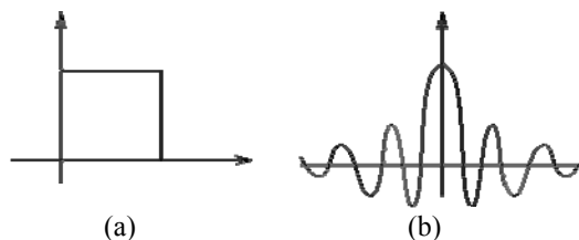
Fig. 3 Transfer function for an ideal low pass filter (a) Frequency domain components (b) spatial domain components.
