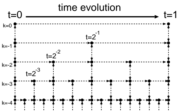
Fig. 2. Schematic view of time evolution for hierarchical individual timestep method. All nodes have individual time on • of this figure, and update when they quantize with global time t . Here, the condition for the change of \Delta t_i is defined by Eq.(7)-Eq.(10). Thus, node states can move only on the dotted lines.
