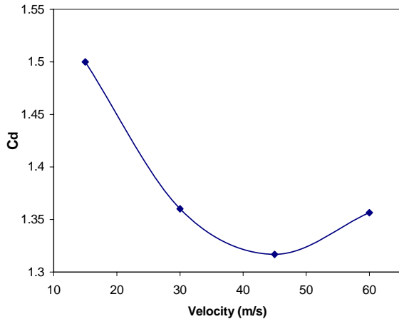
Fig. 5 Variation of drag coefficient ( C_d ) with Velocity
