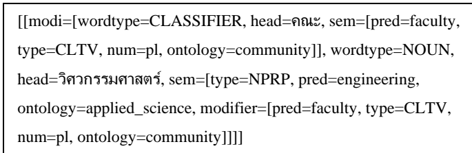
Fig. 2 An example of the output resulting from syntactic analysis
