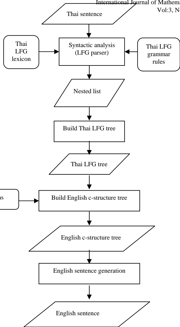
Fig.1 The Architecture of the system
