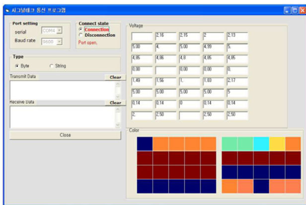
Fig. 3 Software program
