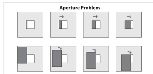
Fig. 5 Aperture problem
