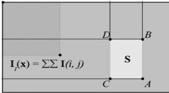
Fig. 1 Integral Image
