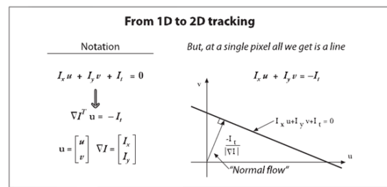
Fig. 4 Normal Flow
