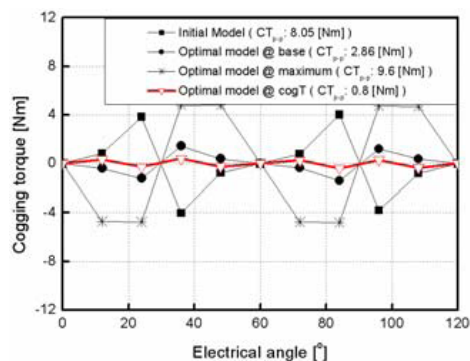
Fig. 10 Cogging torque comparison of each model
