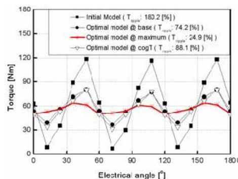
(b) @ Maximum speed
