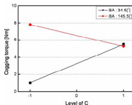
(c) Cogging torque
