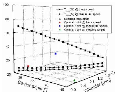
Fig. 8 Variation of each response according to design factors (SO: 8.68 mm)
