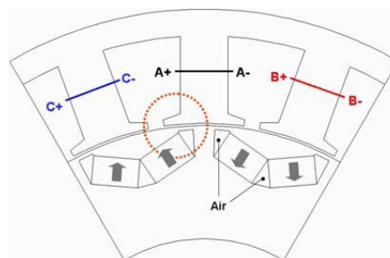
Fig. 1 Configuration of initial designed IPMSM
