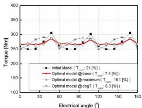
(a) @ Base speed
