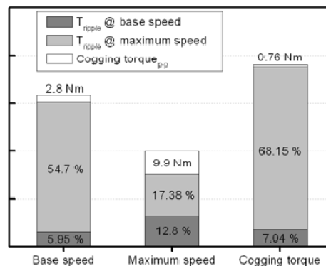
Fig. 7 Characteristics in optimal model of each response
