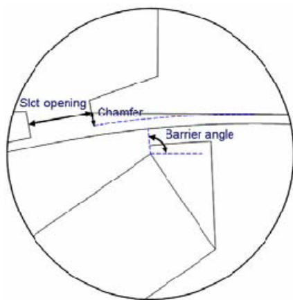
Fig. 5 Design variables for optimization
