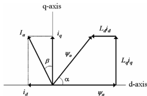
Fig. 4 Phasor diagram of IPMSM
