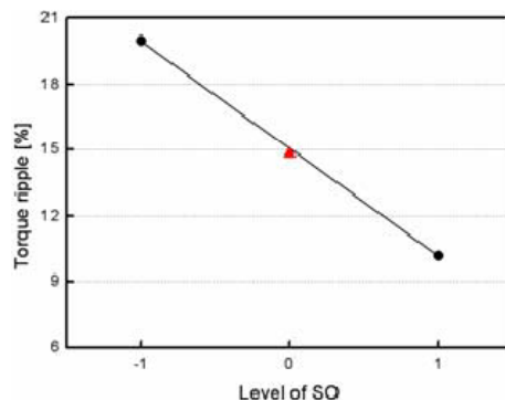
(a) Torque ripple @ base speed
