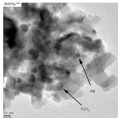
Fig. 4 TEM images of TiO 2 films after immerse in 0.1 M of AgNO 3 solution and then exposed UV for 120 minute.
