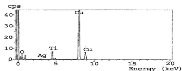
Fig. 3 EDX image of the Ag nanoparticles with UV exposed 120 min on TiO 2 films.
