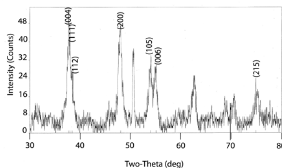
Fig. 5 XRD of the Ag nanoparticles on TiO 2 film having a Face Centered Cubic structure.
