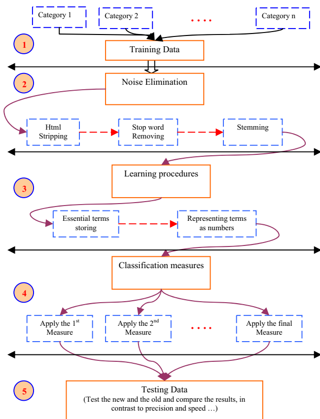
Fig. 1: The stages of the fuzzy similarity approach.
