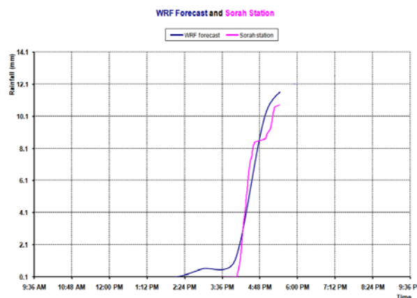
Fig. 10 WRF model results versus real rainfall measurements
