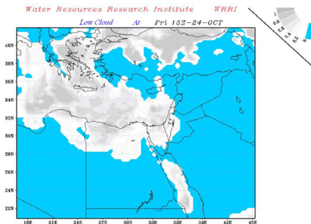
Fig. 7 The cloud pattern over Egypt in October 24 th , 2008
