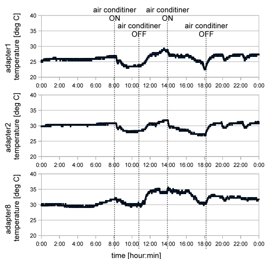
Fig. 10. Air temperature from sensors on layout A
