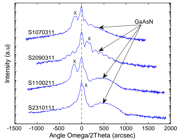
Fig. 3 XRD rocking curves after removal of the InGaAs/GaAs MQW.
