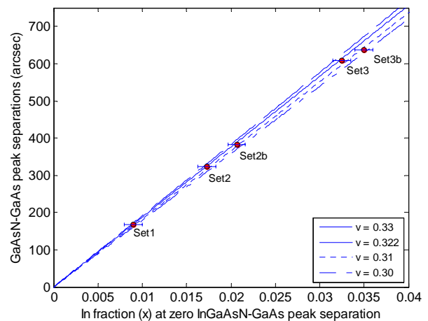
Fig. 6 Plot of GaAsN-GaAs peak separations versus In fraction x .
