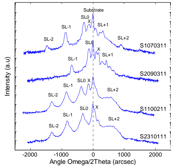
Fig. 2 XRD rocking curves.
