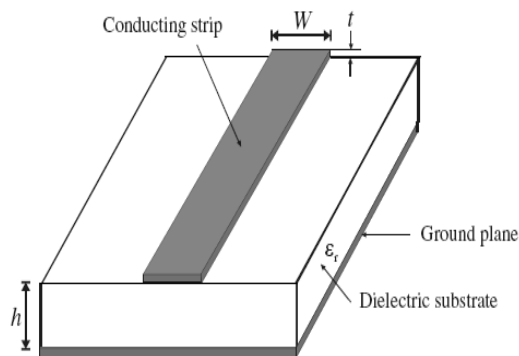
Fig. 1 General Microstrip structure
