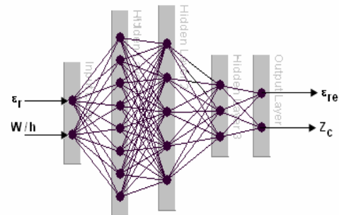
Fig. 3 Neural model for Microstrip Analysis
