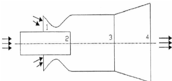
Fig. 3 Schematic view of a supersonic ejector
