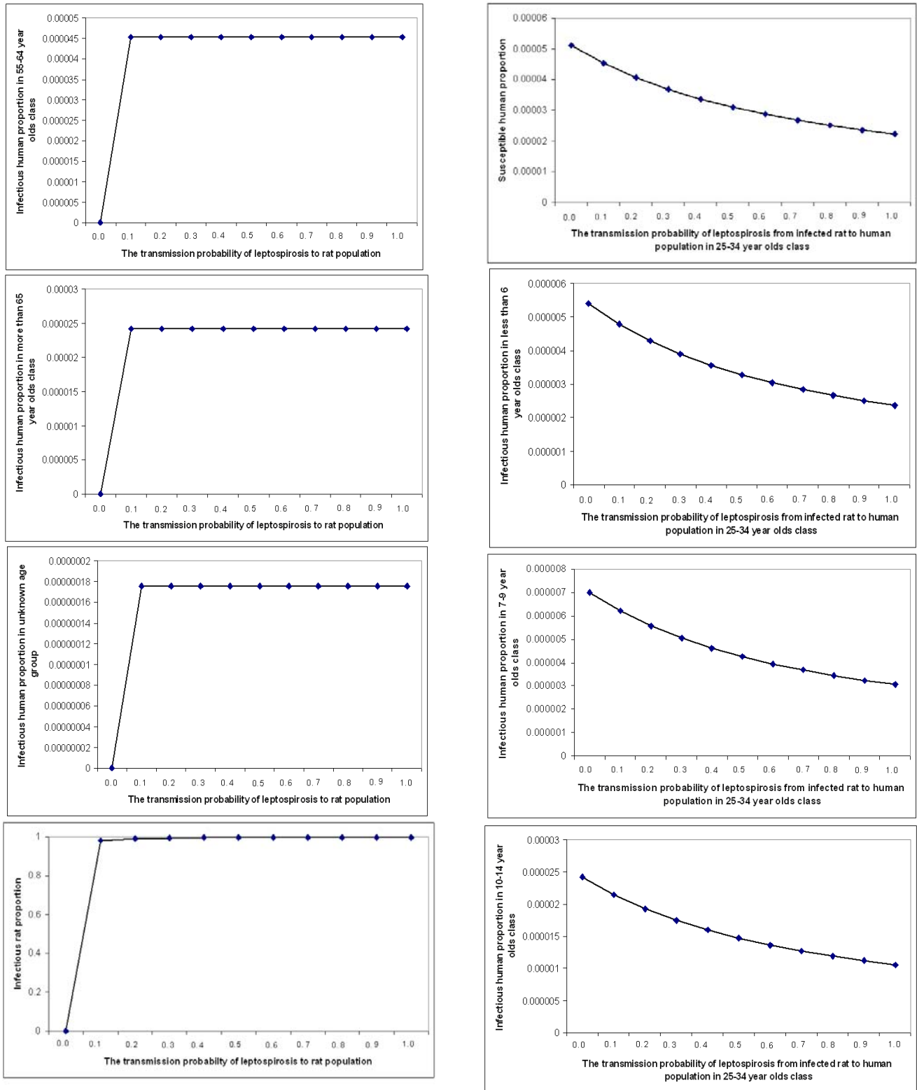
Fig. 1 Bifurcation diagrams of the solutions (4), (5) and (8) for different values of \theta . The value of parameters in the model are shown in Table I
