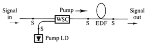
Fig. 1 Forward pumped EDFA structure
