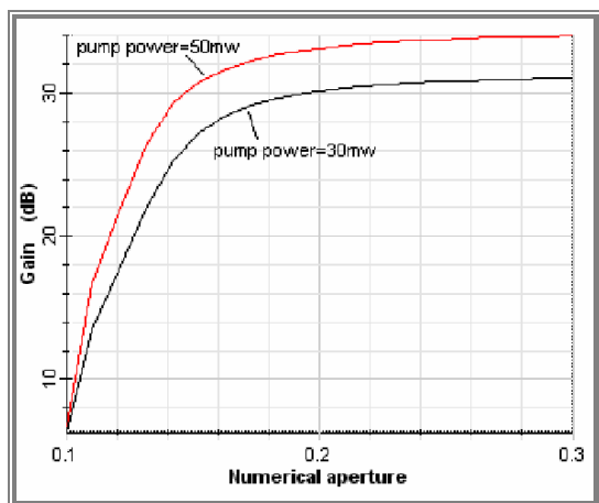
Fig. 6 Signal gain as a function of NA
