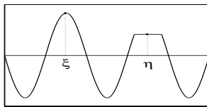
Fig. 4. Two kinds of the intrinsic maximum points.
