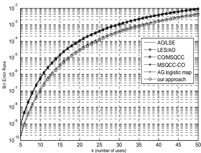
Fig. 3 variation BER via K for SNR=15 and N=127
