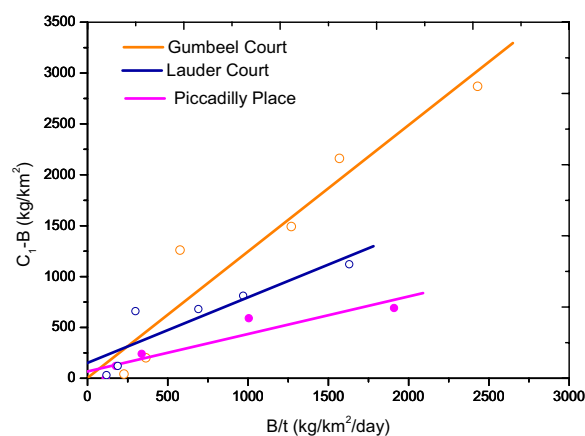
Fig. 8. Saturation Function Build-up Parameters Estimation (Road Surfaces)
