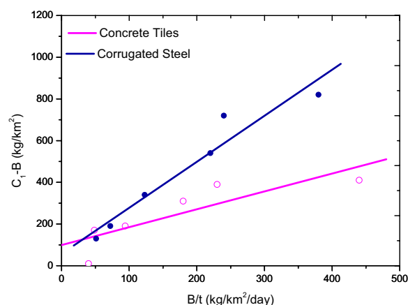
Fig. 9. Saturation Function Build-up Parameters Estimation (Roof Surfaces)
