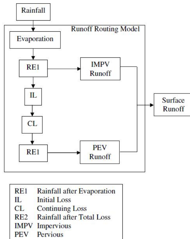
Fig. 1. Structure of the Runoff Model adopted in the model
