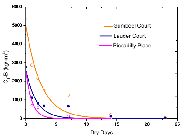
Fig. 6. Exponential Function Build-up Parameters Estimation (Road Surfaces)
