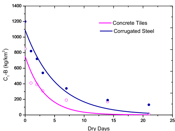
Fig. 7. Exponential Function Build-up Parameters Estimation (Roof Surfaces)
