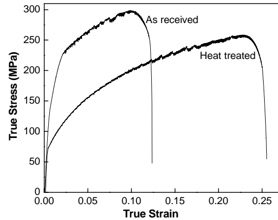
Fig. 3: True stress vs. True strain curve for as received and heat treated sample deformed at a strain rate of 3.8 \times 10^{-4} \text{ s}^{-1} .
