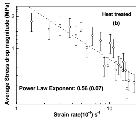
Fig. 6: Variation of average stress drop magnitude for (a) as received and (b) heat treated sample.
