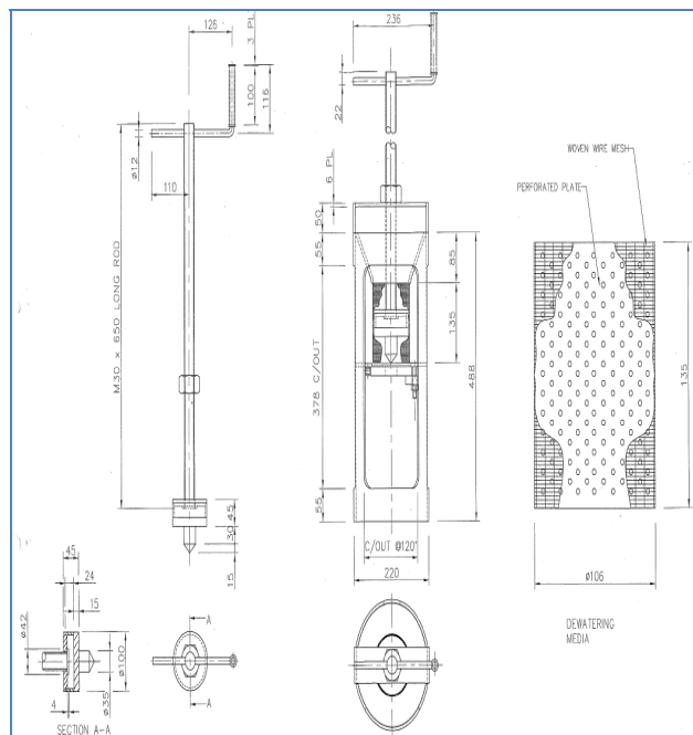
Fig. 3 General arrangement drawing of the screw press
