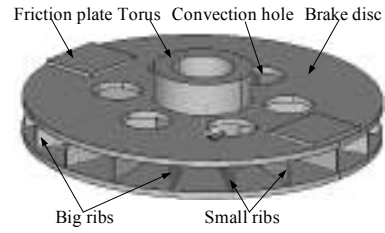
Fig. 2 Disc brake device
