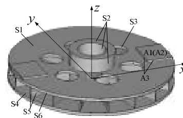
Fig. 1 Three-dimensional model of disc brake
