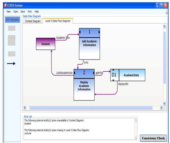
Fig. 3 Example of Level 0 Data Flow Diagram
