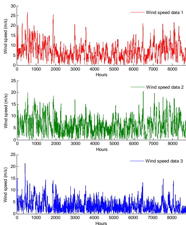
Fig. 1. Wind speed data
