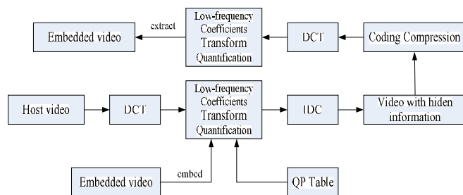
Fig.2 The design framework of Video in Video
