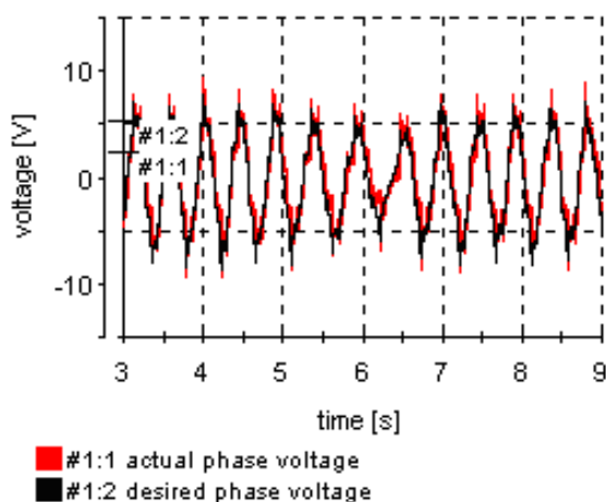
Fig. 16 Desired and actual phase voltage with compensation
