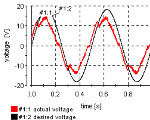
Fig. 10 Actual and desired phase voltage without compensation of dead time
