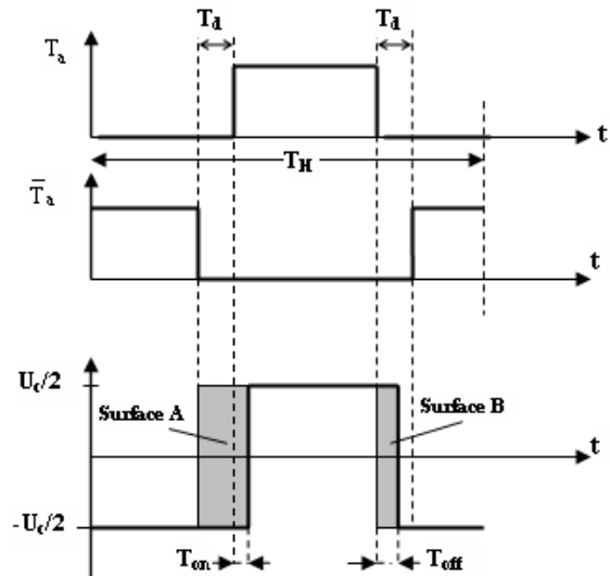
Fig. 4 Pole voltage error \Delta V'_{a0} for i_{as} > 0
