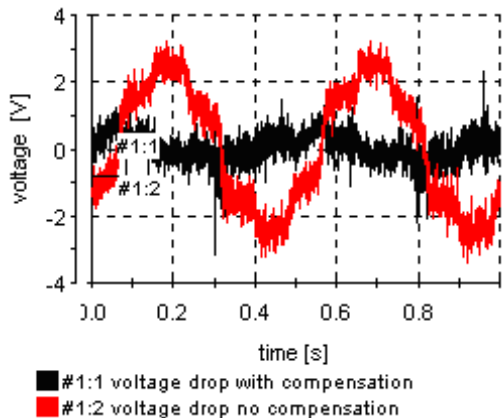
Fig. 9 Phase voltage drop \Delta V_m without and with compensation
