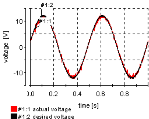
Fig. 8 Actual and desired phase voltage with compensation
