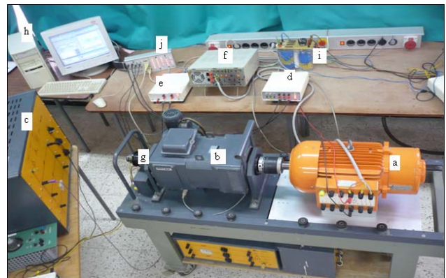
Fig. 6 Photo of the experimental system: (a: induction machine, (b,c): system of load, (d,e): current and voltage transducers, f: IGBT based-inverter, g: incremental coder, h: PC including dSPACE card, i: three-phase rectifier and capacitive filter, j: dSPACE external panel
