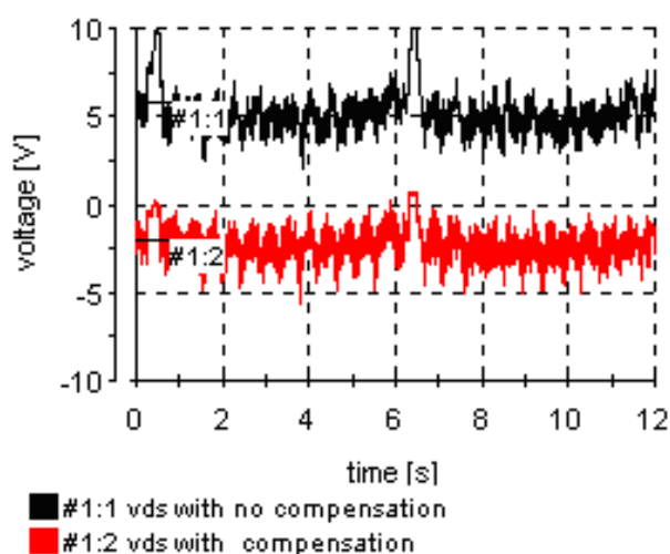
Fig. 17 Reference voltage V_{ds} with and without compensation
