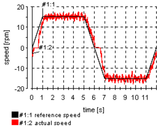
Fig. 13 Speed inversion without compensation
