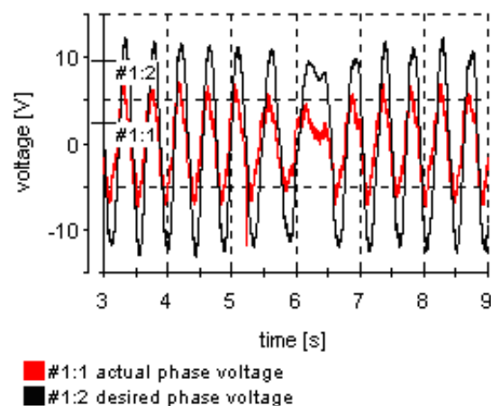
Fig. 15 Desired and actual phase voltage without compensation
