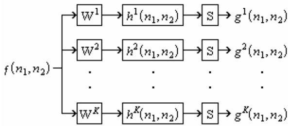
Fig. 1 Observation model
