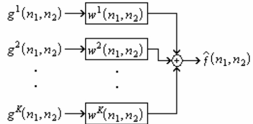
Fig. 2 Reconstruction stage
