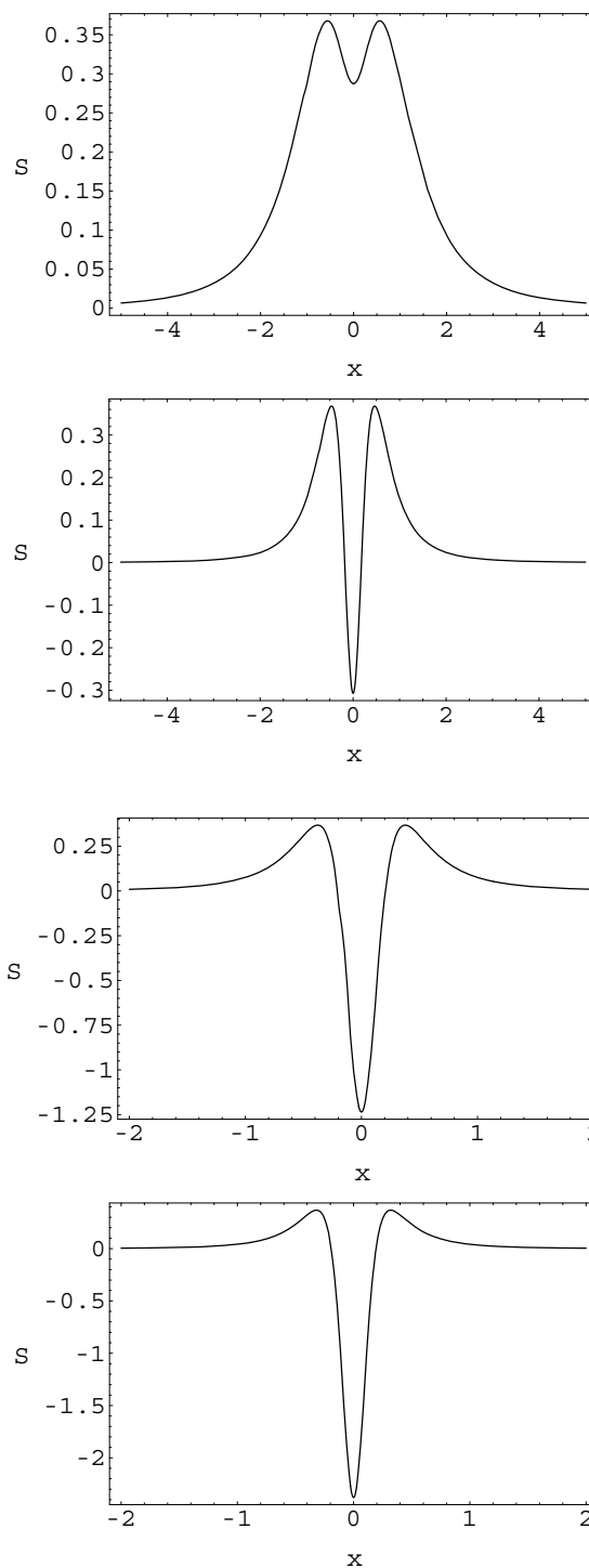
Fig. 2. Momentum space information densities of hydrogen potential for (a) n = 1 , (b) n = 2 , (c) n = 3 and (d) n = 4 .
