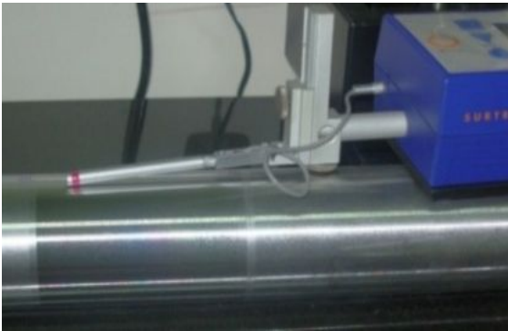
Fig. 6 Surface Roughness Measurement
