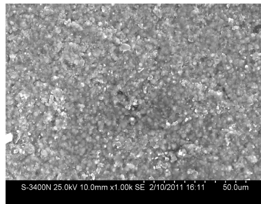
Fig. 2 FESEM photo of the powder
